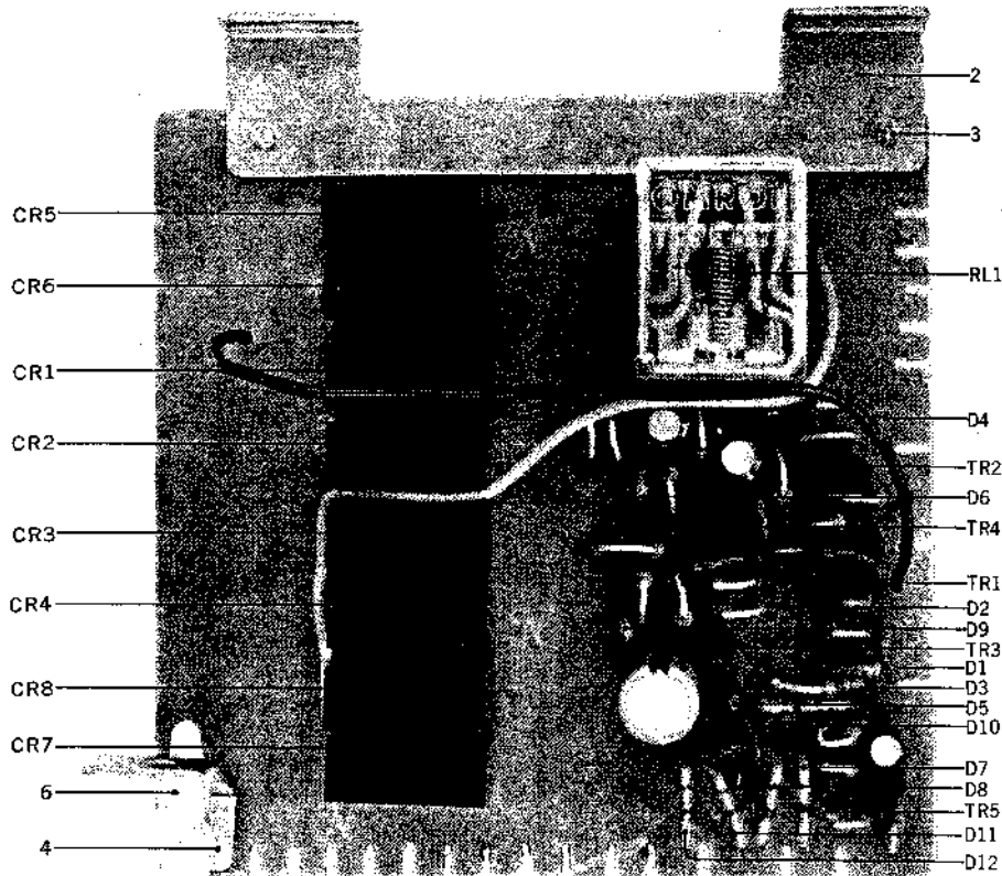
FIG. 7 PHOTO OF SYSTEM CONTROL P.C. BOARD (MU-1202)
