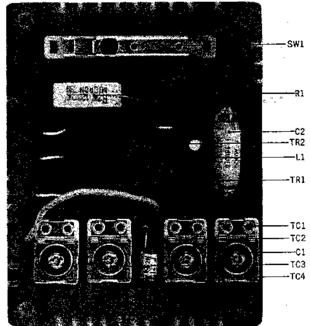
FIG. 12 PHOTO OF OSC. P.C. BOARD (MU-5242)
