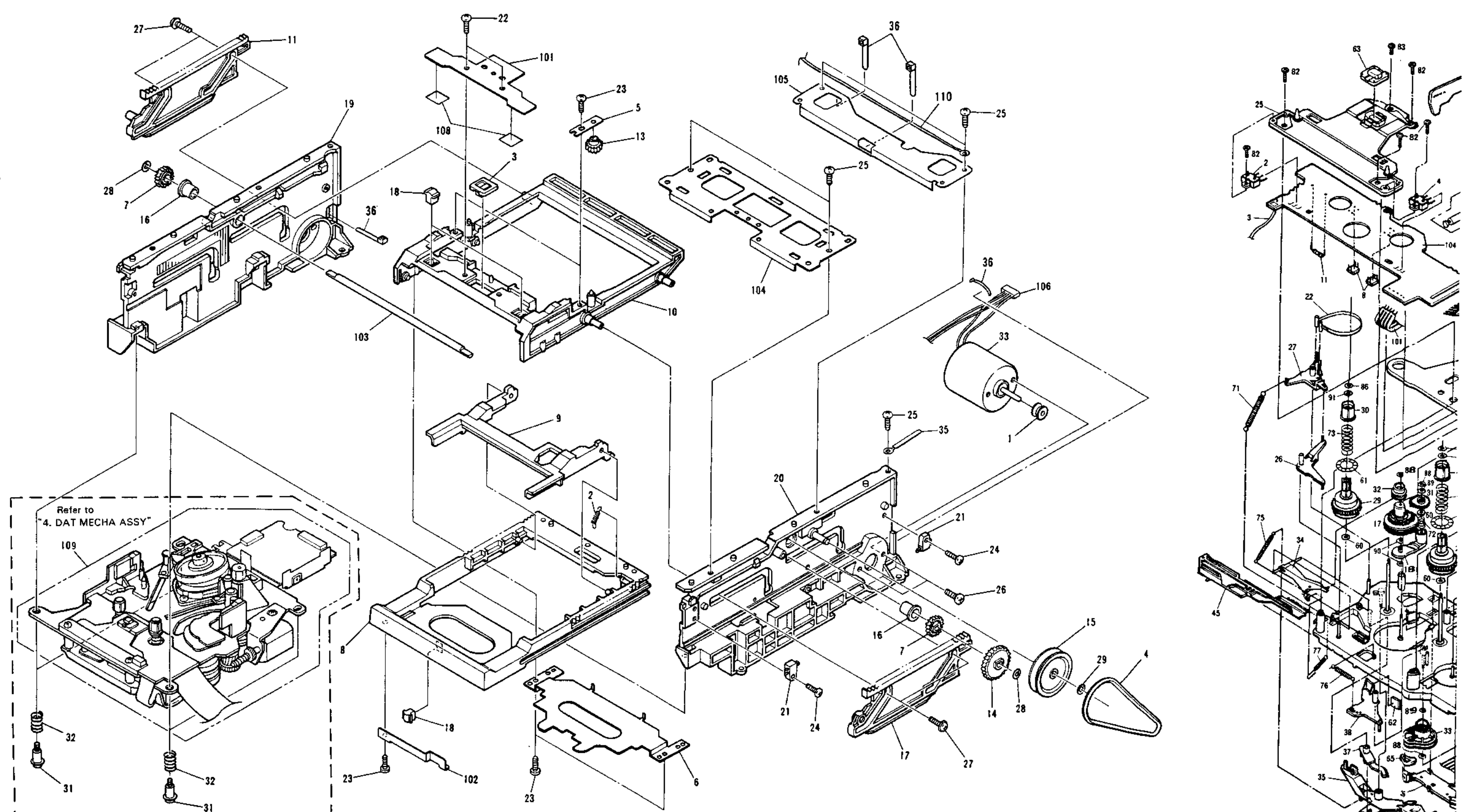
EXPLODED VIEW-3 (CASSETTE INSTALLATION UNIT)
