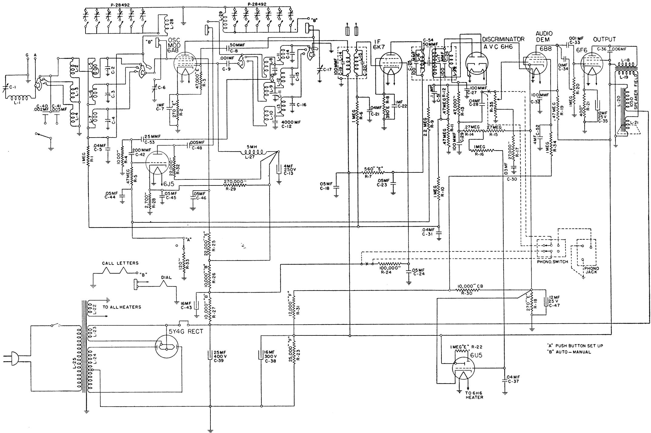
Fig. 3. Schematic Circuit of Receiver.
