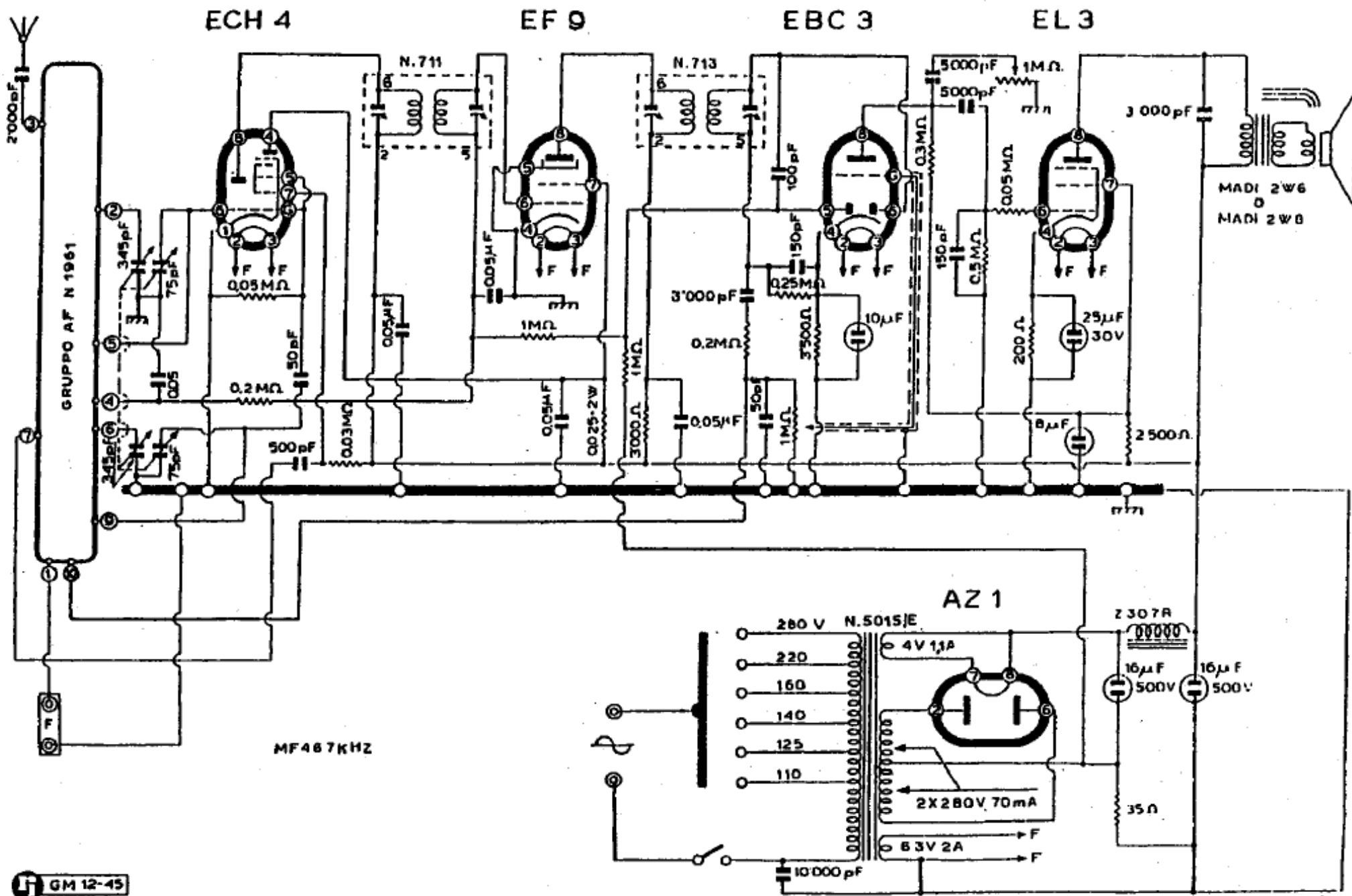
GELOSO S.A. - Mod. Super G 76/RE
