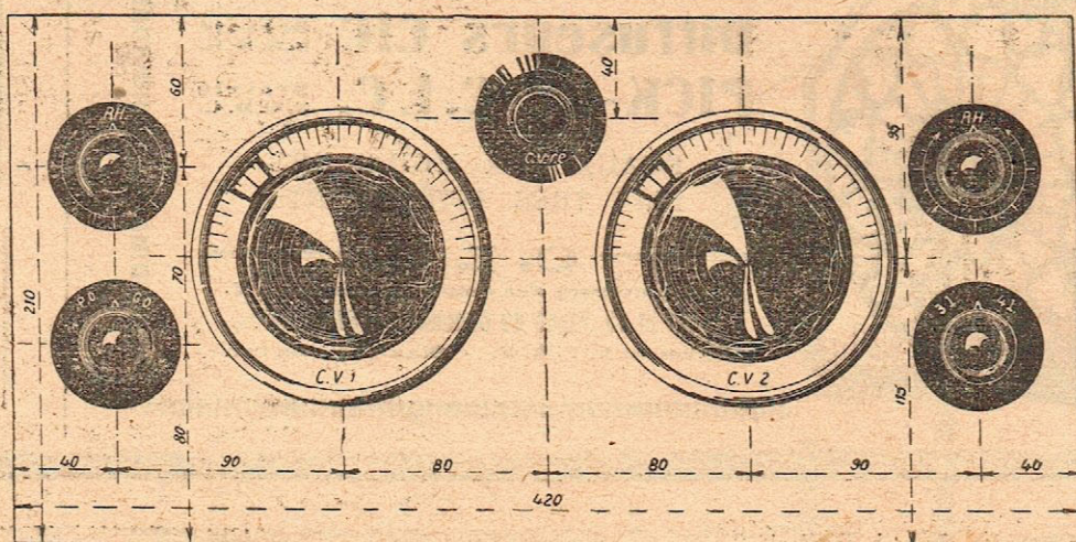
SUPRA-PERFECT. (Vue avant)
