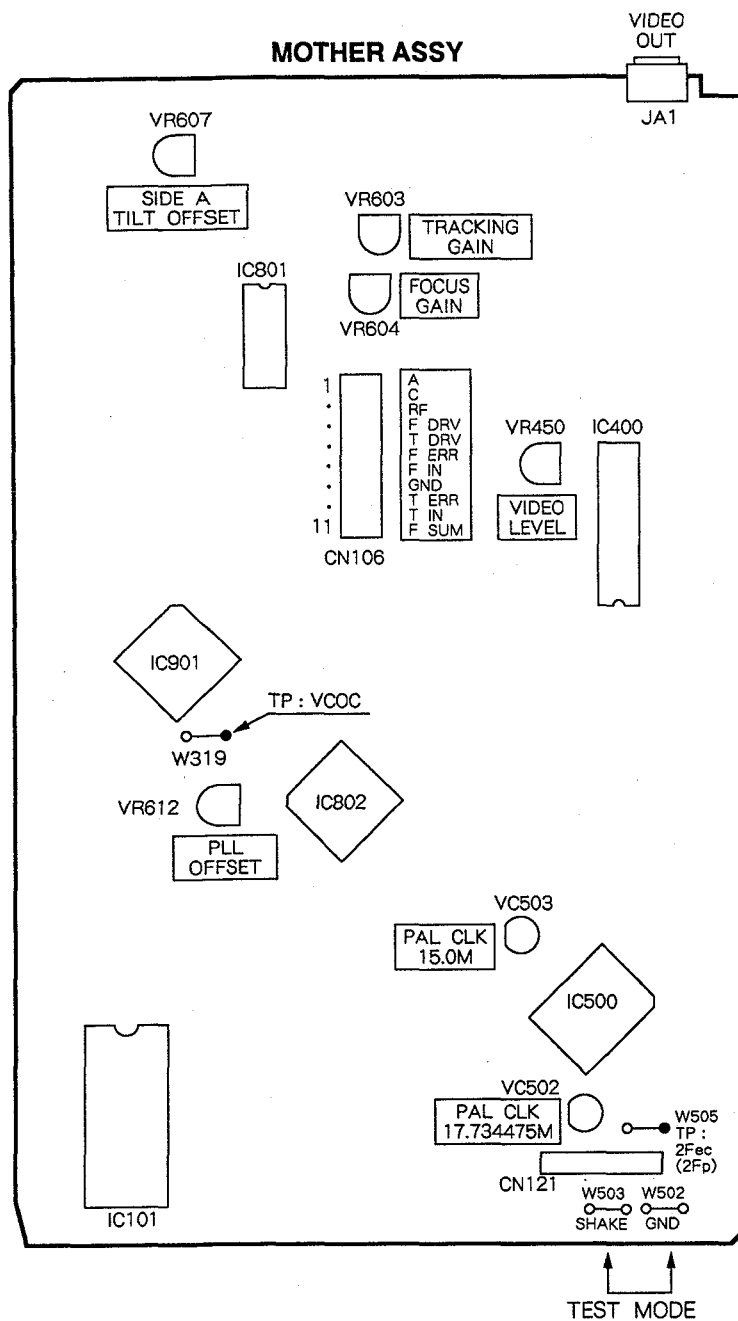
Fig. 14 Adjustment diagram of MOTHER assy
