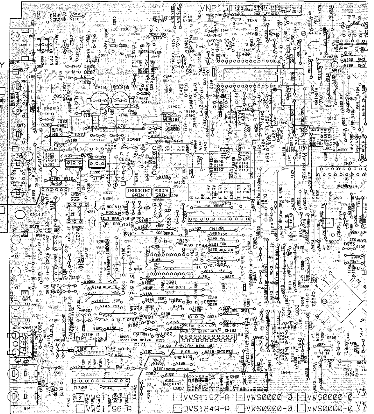
MOTHER ASSY
